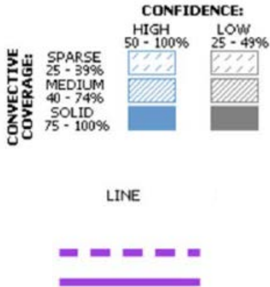
Figure 9-2. CCFP Forecast Convective Coverage
